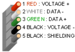
1X5 HEADER CONNECTOR
