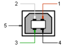
USB TYPE B FEMALE PANEL MOUNT
