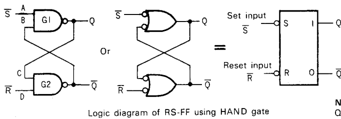
Logic diagram of RS-FF using NAND gate
