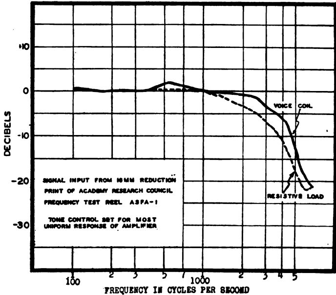
FIGURE 14.—Response-frequency characteristic of amplifier, including scanning beam. Projector F.
