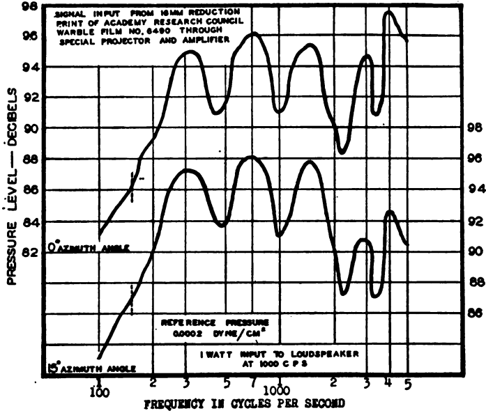
FIGURE 23.—Response-frequency characteristic of loudspeaker. Projector B.
