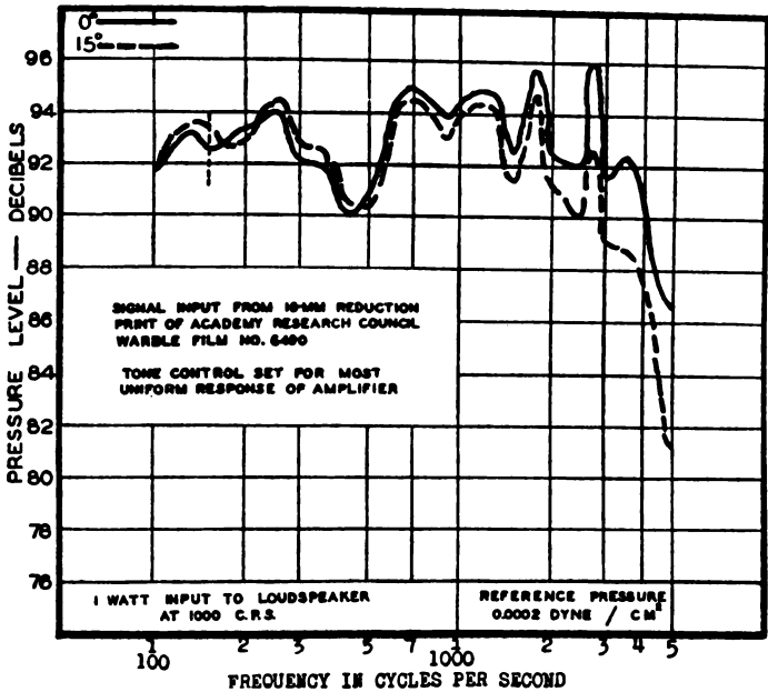
FIGURE 2.—Over-all response-frequency characteristic of projector sound-reproducing system.
