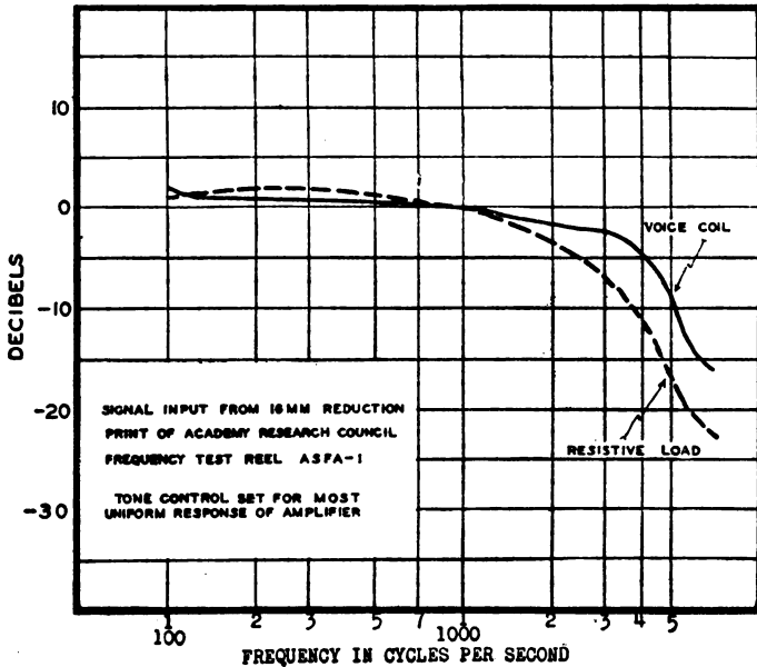
FIGURE 9.—Response-frequency characteristic of amplifier, including scanning beam. Projector A.
