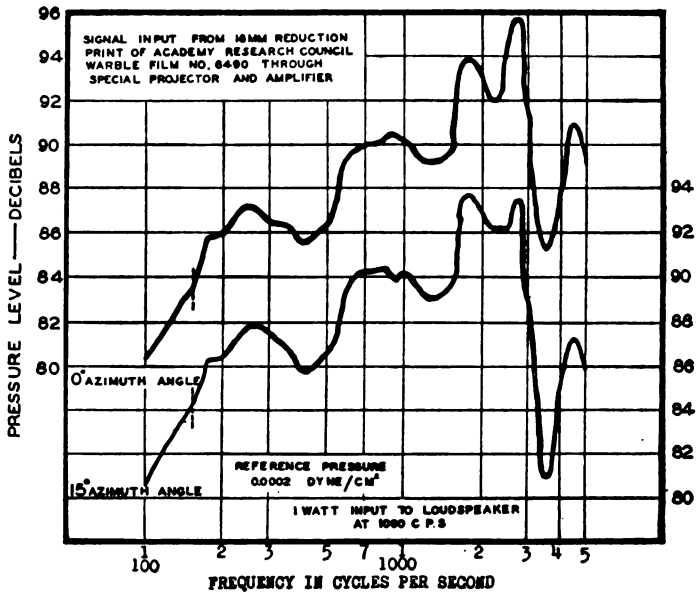
FIGURE 25.—Response-frequency characteristic of loudspeaker.
