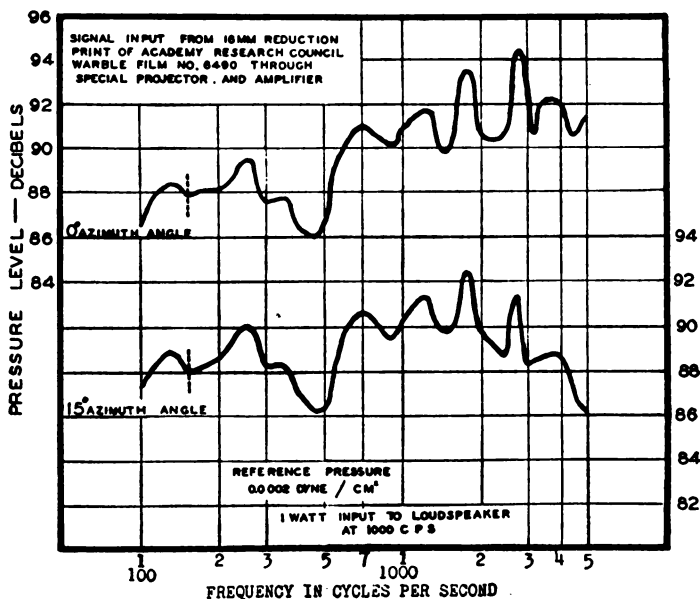
FIGURE 22.—Response-frequency characteristic of loudspeaker.
