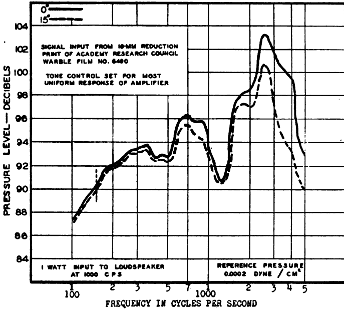
FIGURE 4.—Over-all response-frequency characteristic of projector sound-reproducing system.
