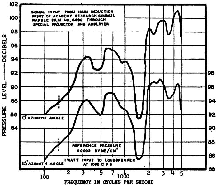
FIGURE 27.—Response-frequency characteristic of loudspeaker.
