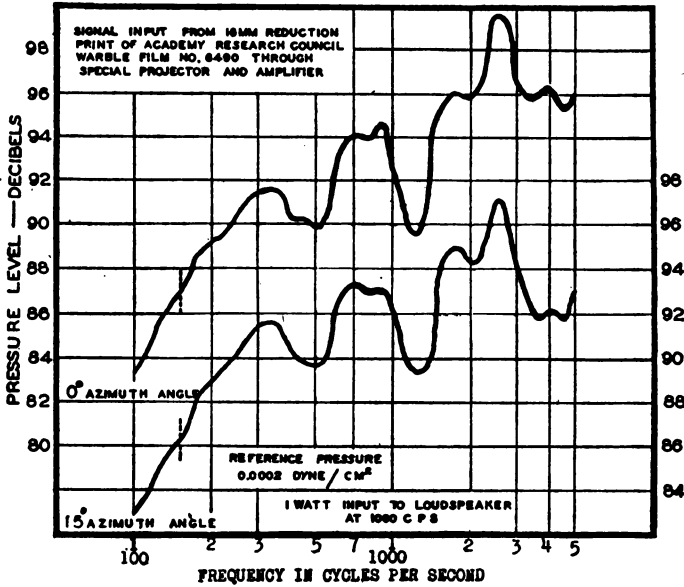
FIGURE 24.—Response-frequency characteristic of loudspeaker. Projector C.
