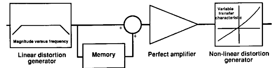
Figure 2 : The new model of an audio amplifier
