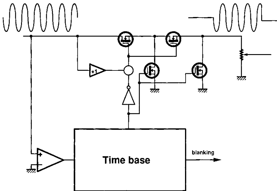
Figure 4 : Generation of the test tone-burst.
