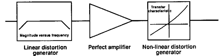
Figure 1 : The classical model of an audio amplifier
