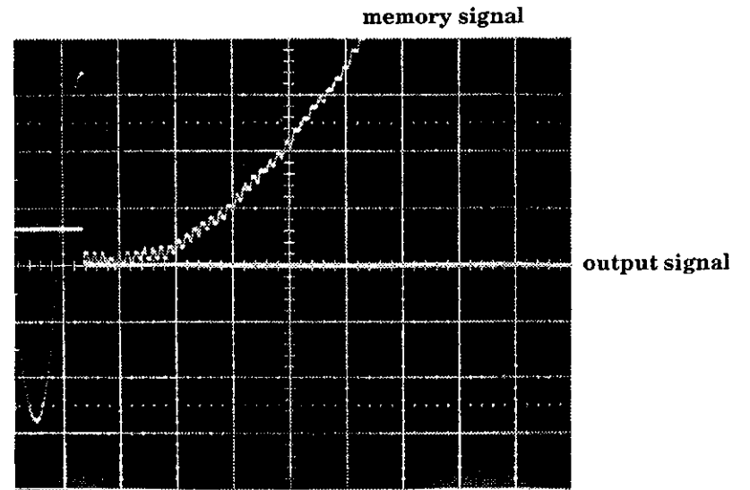
Figure 9 : Output signal ( 2V/div. ) and memory signal ( 2 mV/div. ) for a tube amplifier. Time scale is 10 ms/div. The curvature is induced by a second low-frequency pole.
