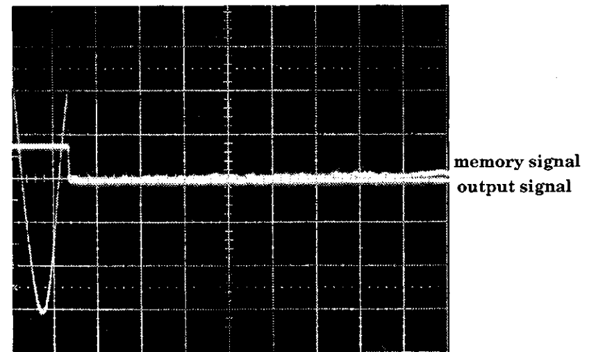
Figure 10 : Output signal ( 2V/div. ) and memory signal ( 0,5 mV/div. ) for a transistor amplifier using a new memory free technology. Time scale is 10 ms/div.
