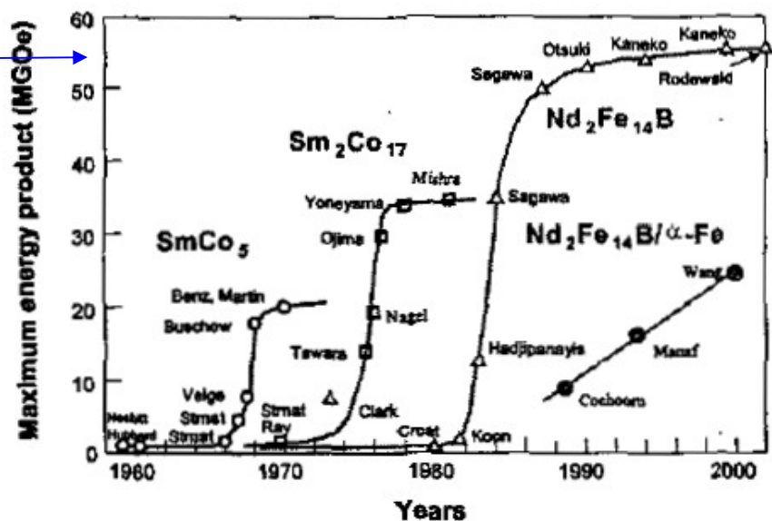
Developments in rare-earth magnets over the years ( Prof. S. Liu, University of Dayton)
