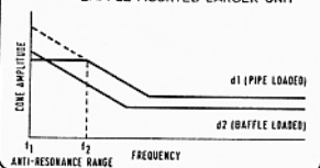
FIG. 3 BASIC CURVES COMPARING SMALL PIPE-LOADED BASS UNIT WITH BAFFLE MOUNTED LARGER UNIT
