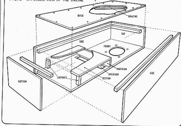
FIG. 5 EXPLODED VIEW OF THE DALINE
