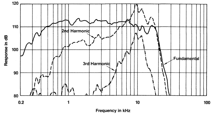
Figure 9A: 2445J and 2360. Distortion raised 20 dB. 6.3 Volts at 1 kHz
