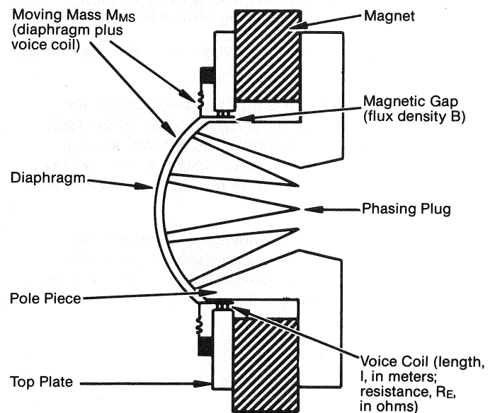
Figure 1: Details of a Compression Driver
