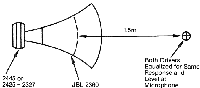
Figure 8: Test Set-up for Driver Comparison
