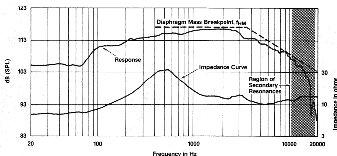
Figure 6: Response of JBL 2425 Driver on 25.4mm (1 in) PWT with 1 Milliwatt Input
