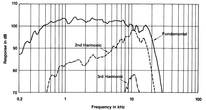
Figure 9B: 2445J and 2360. Distortion raised 20 dB. 2 Volts at 1 kHz
