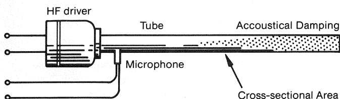
Figure 5: Details of a Plane Wave Tube
