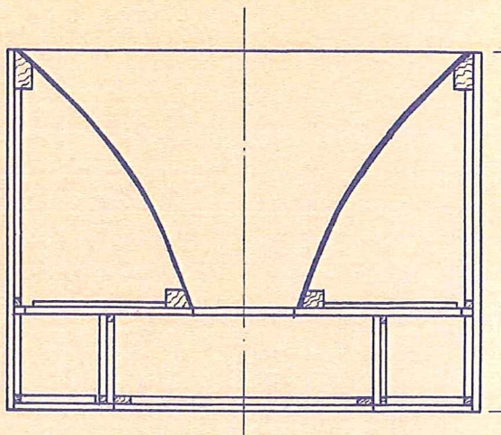
SECT B-B
