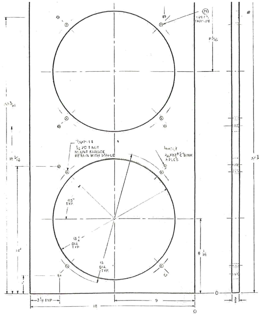
SPEAKER MOUNTING BOARD
