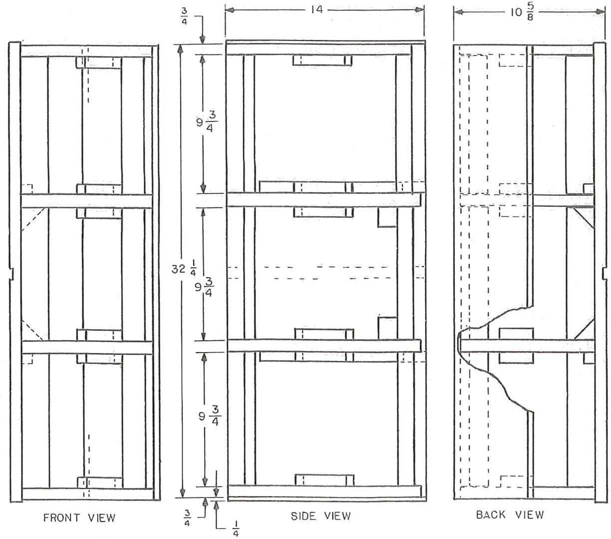
SPEAKER MOUNTING BOARD
