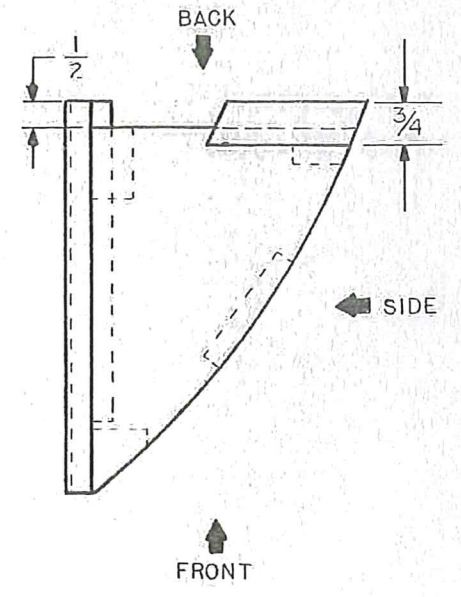
HORN SIDE ASSEMBLY
