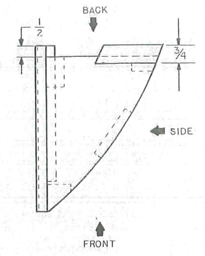
HORN SIDE ASSEMBLY
