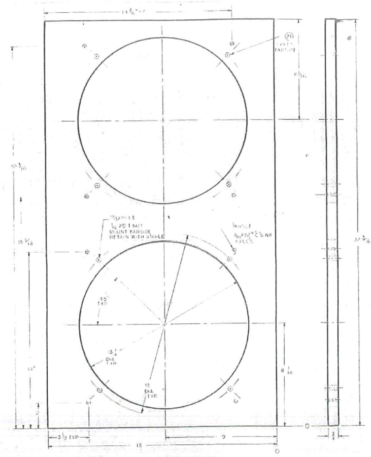
SPEAKER MOUNTING BOARD
