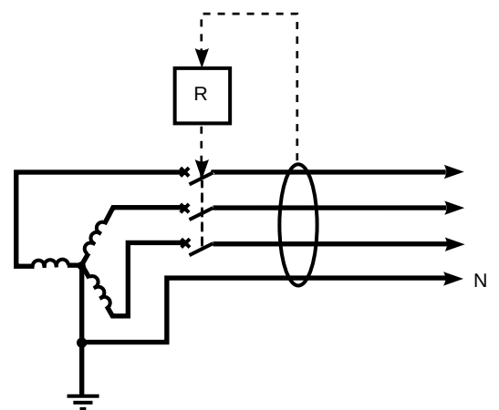
Fig. 16 : zero sequence.
