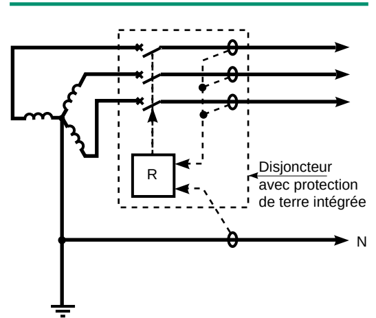
Fig. 14 : residual sensing.
