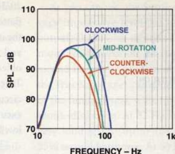
Fig. 1—Frequency response at crossover settings of 33, 55, and 75 Hz.
