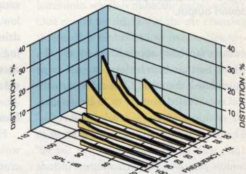
Fig. 3—Harmonic distortion vs. SPL and frequency.
