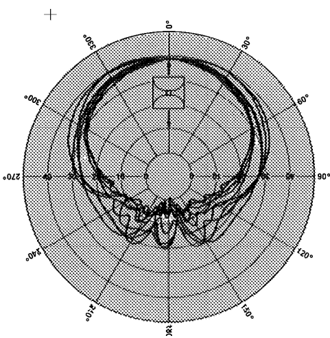
Vertical polar response.
